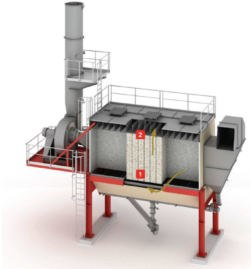
Figure 6: Baghouse Filter
