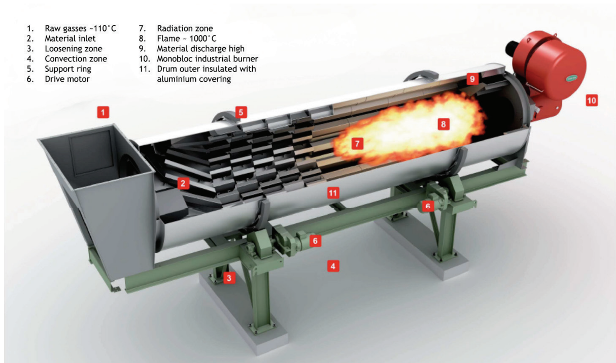
Figure 7: Drying and heating drum
