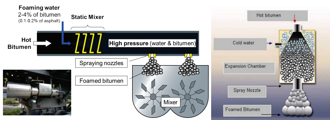
Figures 2: Foaming nozzle www.foamasphalt.info Figures 3: Foaming nozzle [2.]
