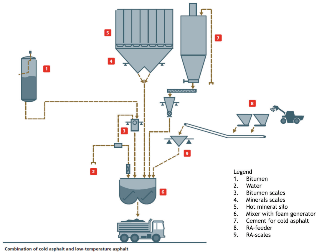
Figure 8: Flow chart of asphalt production with foam bitumen
