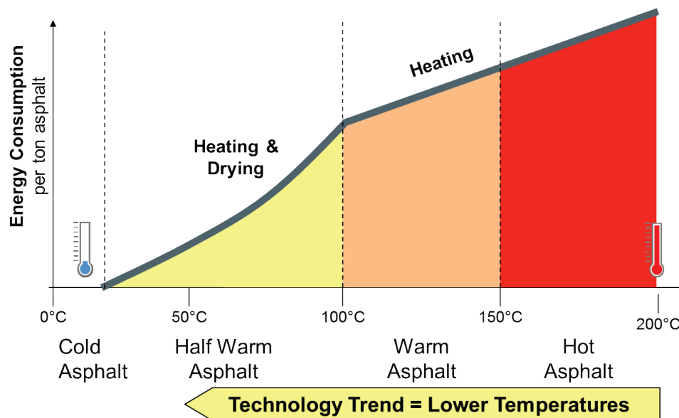
Figure 1: Classification by temperature range
